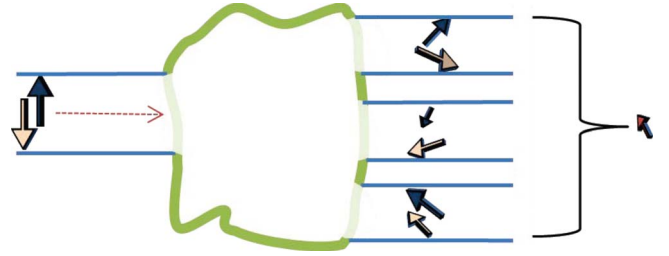
FIG. 2. (Color online) Generic device with one input channel. Unpolarized current, consisting of equal parts spin-up and spin-down components, is incident on a chaotic quantum dot from a single channel on the left. The irregularly shaped region in the middle is a quantum dot in the strong spin-orbit regime. The spin-up incident current has a probability to exit into each of the three channels of the right lead with a different spin direction in each channel, indicated by the direction of the dark arrows. Similarly for the spin-down incident current, indicated by the light arrows. The exit channels are shown spatially separated, for convenience. There is also a probability to scatter back into the left lead (not shown). The total spin current in the exit lead is given by summing the probabilities and directions of the six spin polarizations shown, which is the meaning of Eq. (4) and is indicated by the arrow on the right.
