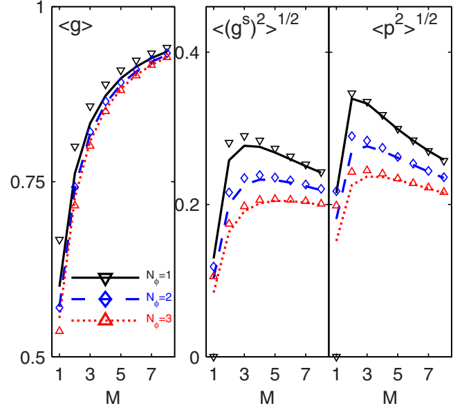
FIG. 4. (Color online) Model with spin-conserving dephasing lead. Numerical (symbols) and analytical (lines) results for normalized mean conductance \langle g \rangle , rms spin conductance g^s , and rms spin polarization p of current exiting a chaotic quantum dot with N=1 channel in the entrance lead. M and N_\phi are the numbers of channels in the exit and dephasing leads, respectively. An average over 60 000 S matrices from the CSE was performed for each data point. The lines are from Eqs. (28) and (29).
