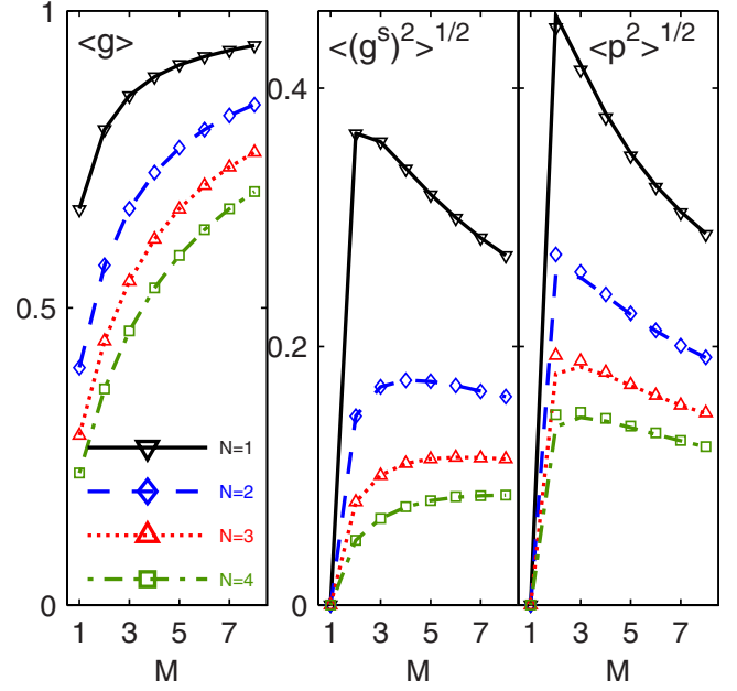
FIG. 3. (Color online) Numerical (symbols) and analytical (lines) results for normalized mean conductance \langle g \rangle , rms spin conductance g^s , and rms spin polarization p of current exiting a chaotic quantum dot with N ( M ) channels in the entrance (exit) lead. An average over 60 000 S matrices from the CSE was performed for each data point. The lines are from Eqs. (19)–(21).
