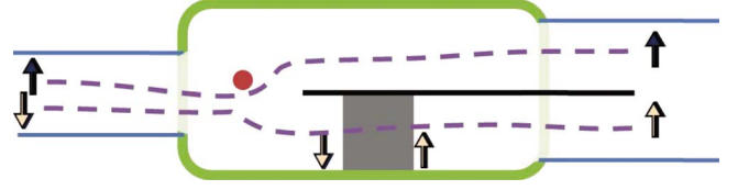
FIG. 1. (Color online) A special model quantum dot with N=1 channels in the left lead and M=2 channels in the right lead. A skew scatterer sends all \hat{z} spins to the top channel and all -\hat{z} spins to the bottom channel. The shaded area in the bottom channel has Rashba spin-orbit coupling of precisely the strength to rotate a down spin at the Fermi energy to an up spin, thus producing a perfectly spin-polarized exit current from any input current, while respecting time-reversal symmetry.
